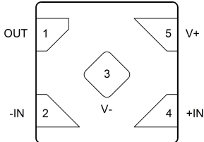
X2SON-5/DFN1x1-5L
