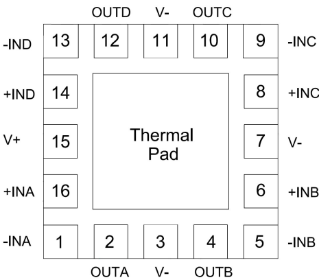
QFN2*2-16L
