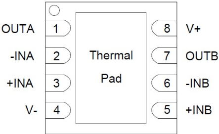
DFN2x2-8L
