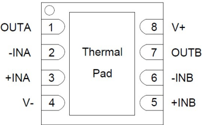
DFN2x2-8L
